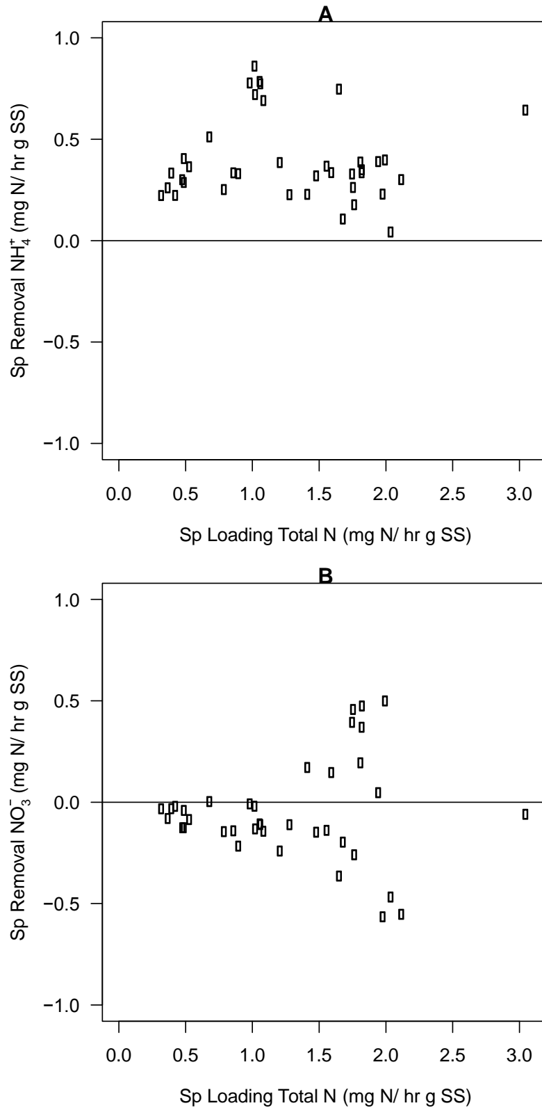
FigureS3: Specific removal rate of (A) \text{NH}_4^+ and (B) \text{NO}_3^- ( \text{mg N hr}^{-1} \text{g SS}^{-1} ) versus specific loading of total N ( \text{mg N hr}^{-1} \text{g SS}^{-1} ).
